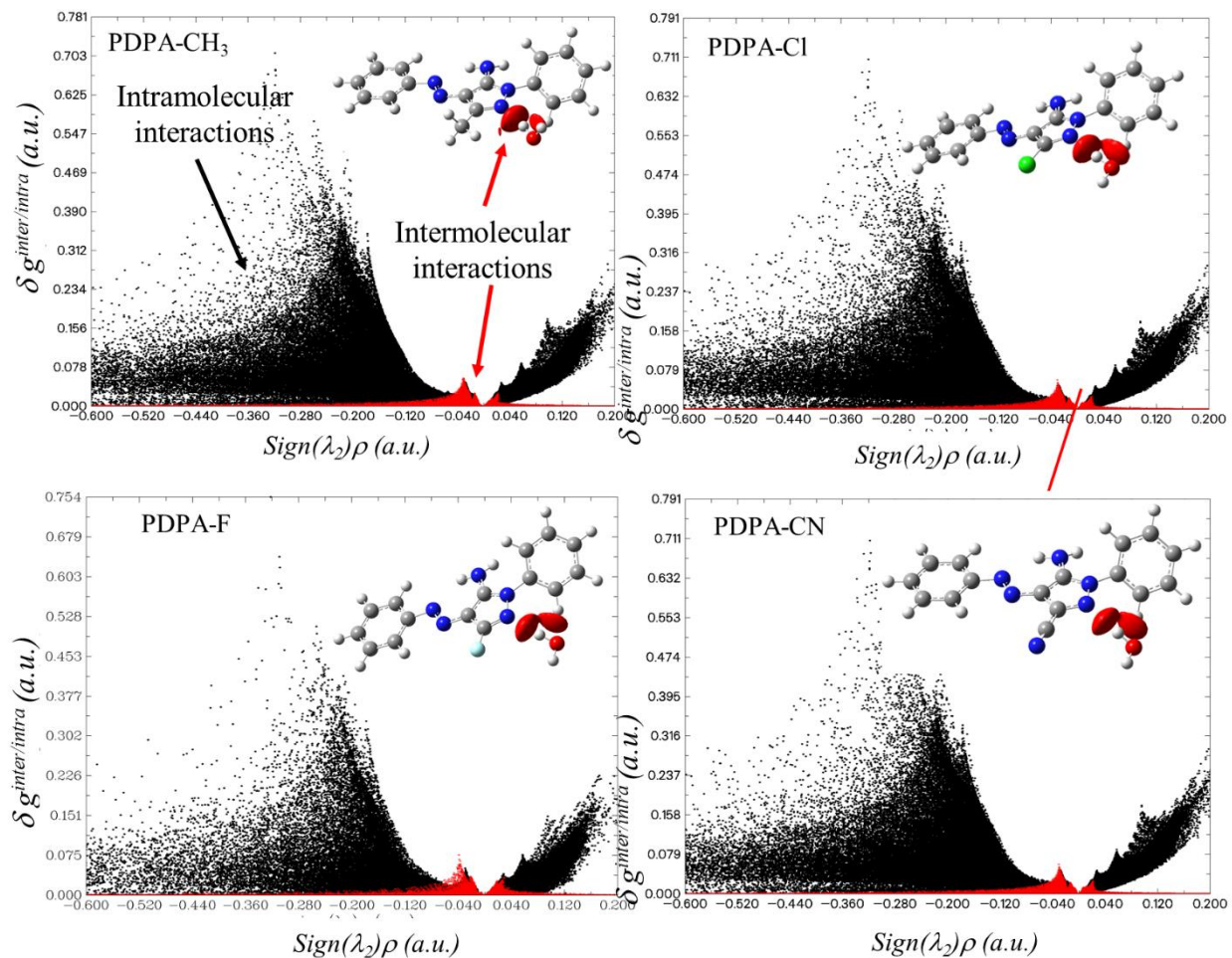
Figure SM3. Scatter plots of \delta g^{inter/intra} (a.u.) versus Sign(\lambda_2)\rho (a.u.) of some PDPA-water complexes, including PDPA-CH 3 .H 2 O, PDPA-Cl.H 2 O, PDPA-F.H 2 O, and PDPA-CN.H 2 O. The corresponding RGD maps are superimposed at the top right of each panel. The red dots correspond to the intermolecular interactions, while the black dots correspond to the intramolecular interactions.
