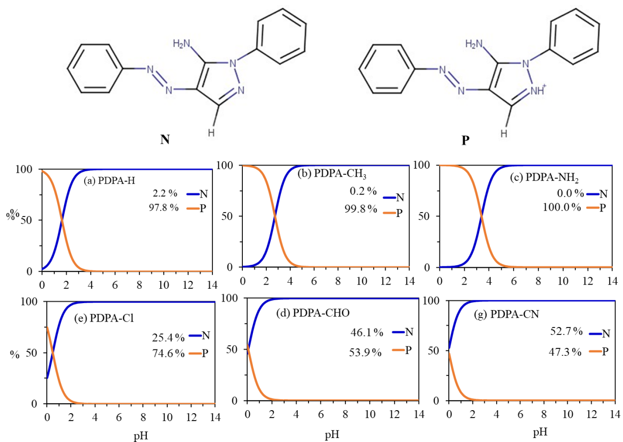
Figure SM1. Relationships between the pH and % possibility of the neutral and protonated forms of the investigated derivatives. For PDPA-F derivative.
