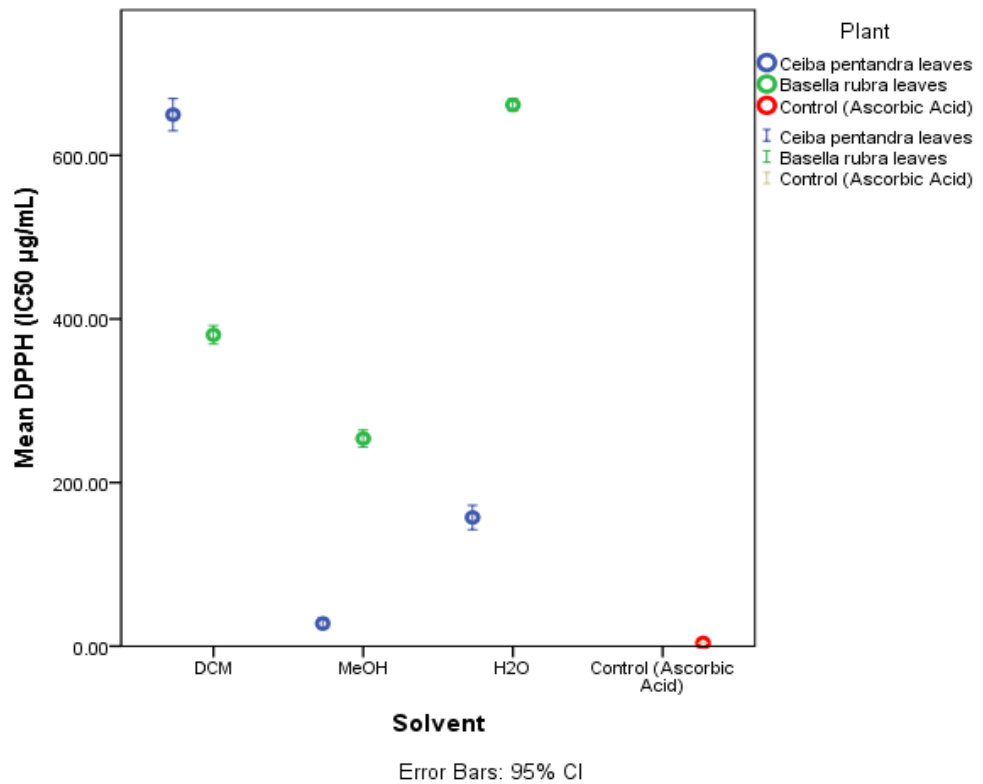
Figure 4b. (Figure 5S) Error bar diagram shows the DPPH assay with the strongest IC 50 value for leaf's methanol extract of Ceiba pentandra close to control (Ascorbic Acid) followed by its aqueous extract.
