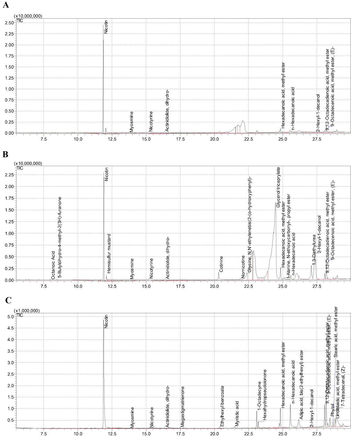
Supplementary Fig S1: Representative chromatograms of naswar sample (S2) in three different external extraction solvents (a) N- Hexane (b) Chloroform (c) Methanol
