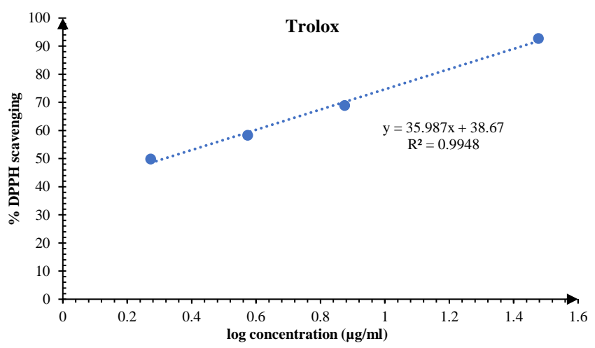
Fig. S 2 Asiaticoside, gallic acid and Trolox calibration curve
