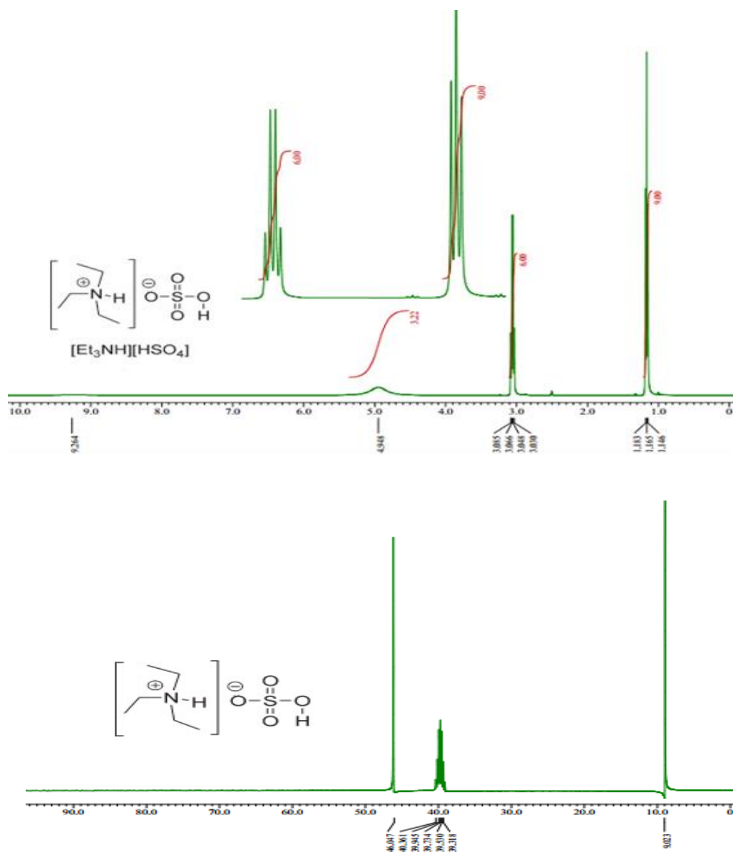
Fig. S 1 1 H-NMR and 13 C-NMR spectrum of triethylammonium hydrogen sulphate, [TEA][HSO 4 ]
