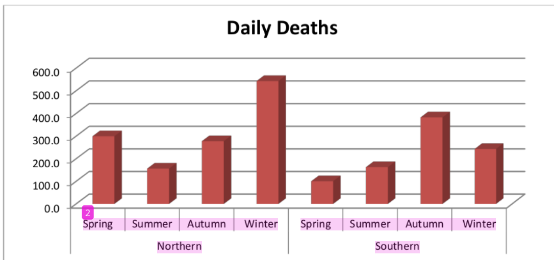
Figure 2: Effect of seasonal variations on the SARS-CoV-2 daily deaths in northern and southern hemisphere countries
