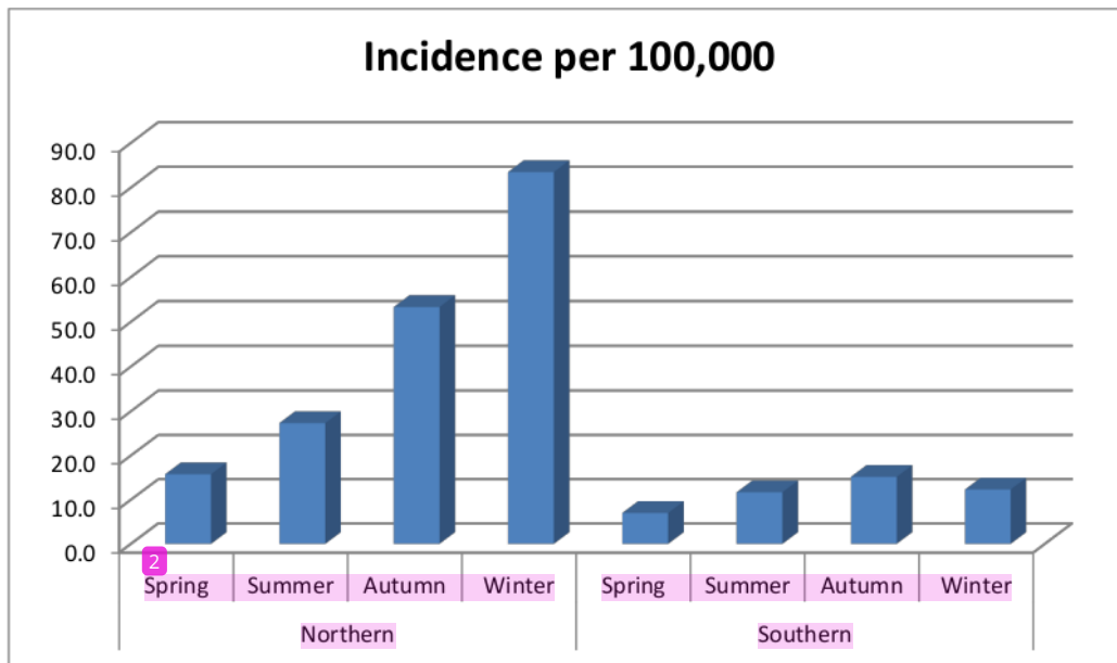
Figure 3: Effect of seasonal variation on the SARS-CoV-2 incidence per 100,000 population in northern and southern hemisphere countries
