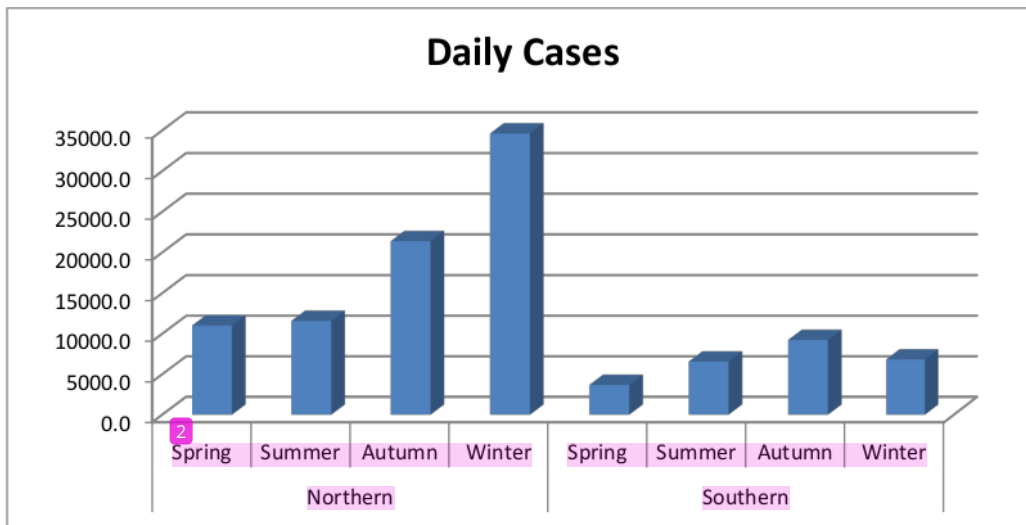
Figure 1: Effect of seasonal variations on SARS-CoV-2 daily cases in northern and southern hemisphere countries
