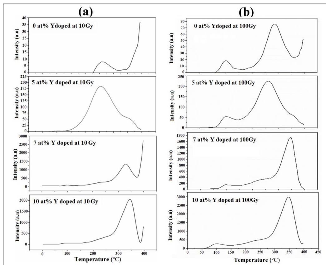
Figure 6: TLD response of Y doped NPs at (a) 10Gy dose (left column) and (b) 100 Gy dose (right column).
