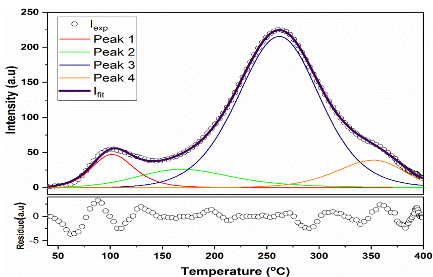
Figure 7: Deconvoluted peak of TLD response for 5 at% Y doped ZnO for 100Gy dose
