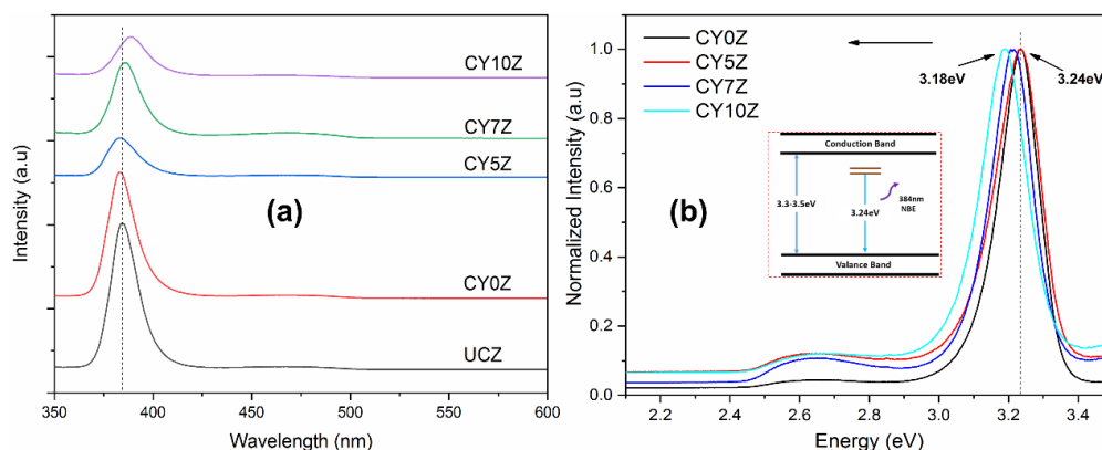
Figure 5. (a) UV-Vis spectra of prepared samples; (b) Bandgap energy plot from PEG-coated samples.
