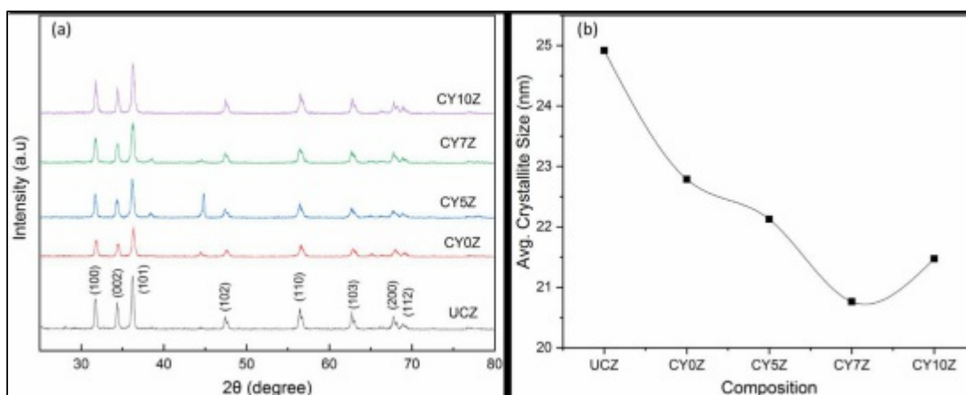
Figure 2: (a) XRD patterns and (b) average crystallite size of uncoated (UCZ), PEG coated Y doped ZnO NPs prepared hydrothermally (CY0Z, CY5Z, CY7Z, and CY10Z )
