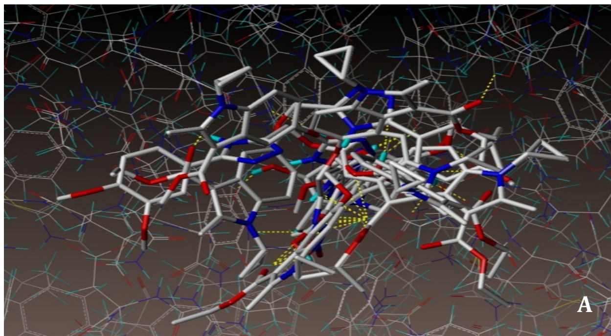
Figure S1 (A-B). Docked view of the compounds 5a-5k at the active site of human Maltase-glucoamylase ( \alpha -glucosidase) protein from human intestine.
