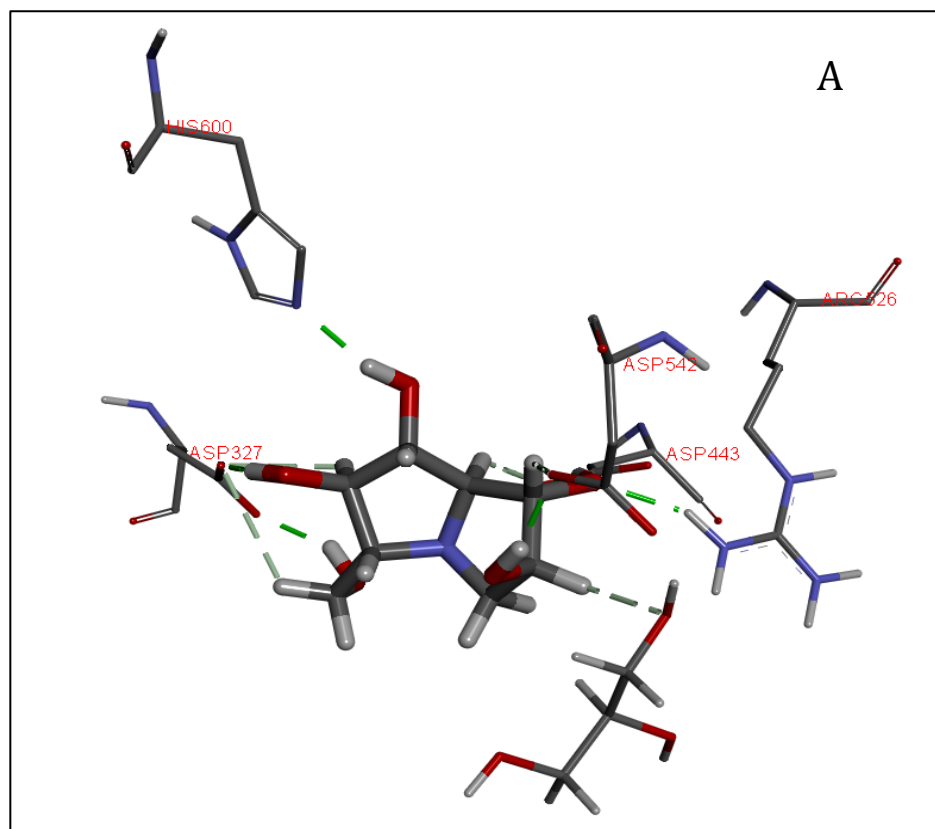
Figure. S2 (A-B). Docked view of ligand, Casuarine at the active site of the enzyme Maltase-glucoamylase ( \alpha -glucosidase) (PDB ID: 3CTT)
