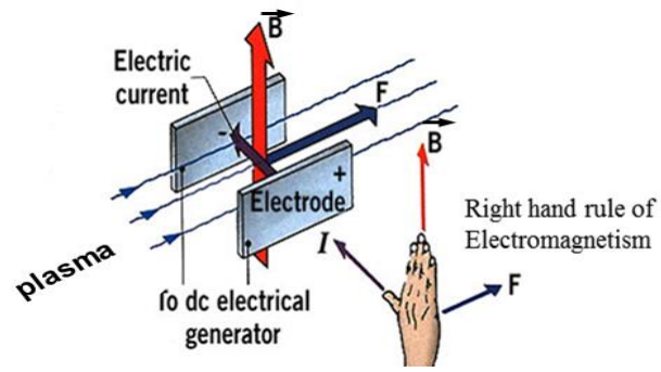
Figure 1 Principle of Magnetohydrodynamics (Masood et al., 2014).
