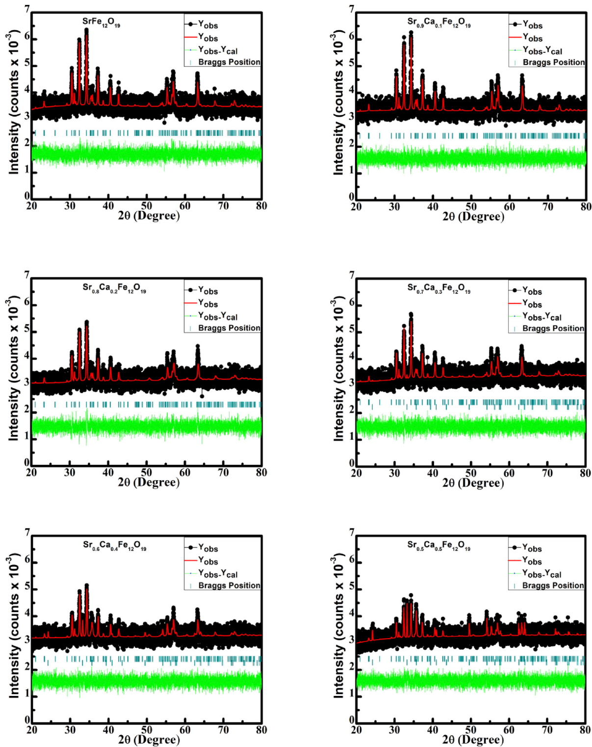
Figure 2. Rietveld refinement of \text{Sr}_{1-x}\text{Ca}_x\text{Fe}_{12}\text{O}_{19} ( x = 0.0-0.5 ).
