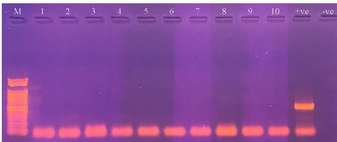
Fig. 3. Agarose gel showing PCR products for the detection of DENV in different mosquito samples (Lanes 1–10). M: DNA marker, +ve: positive control, and -ve: negative control.
