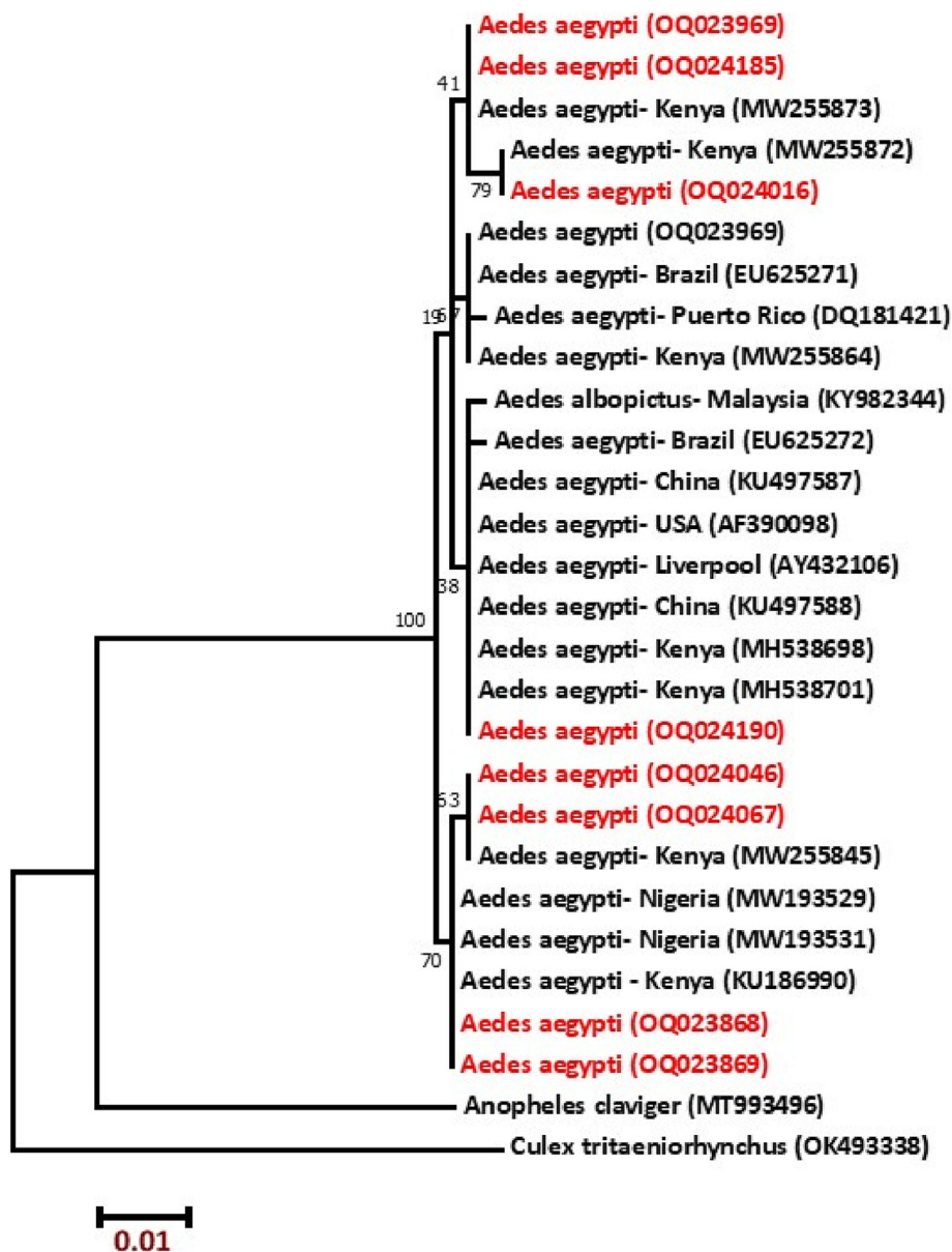
Fig. 2. Molecular phylogenetic analysis of mt COI gene of mosquito specimens by Maximum Likelihood method based on the Tamura-Nei model. The tree with the highest log likelihood (-1147.40) is shown.
