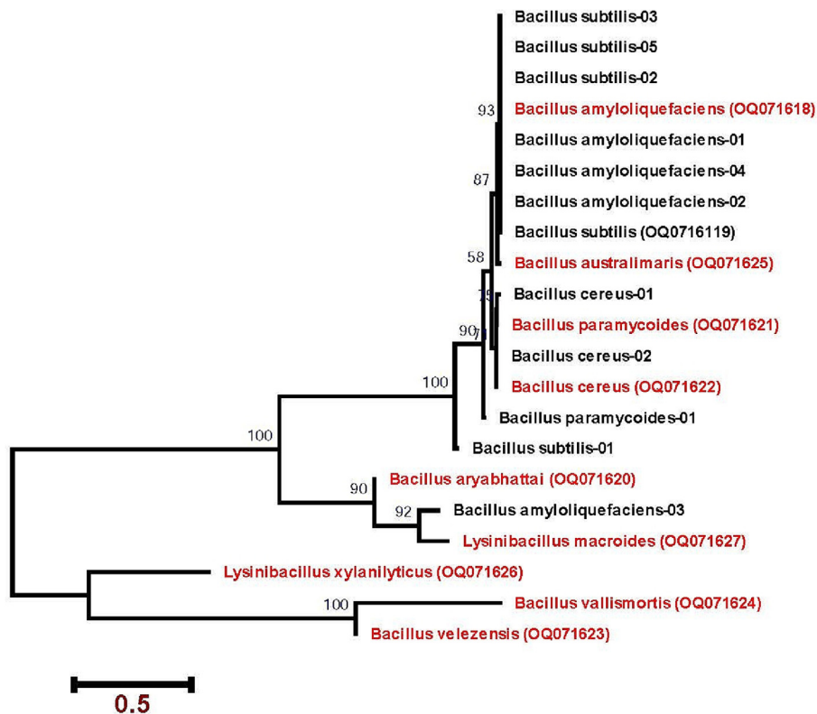
Fig. 6. Neighbor-joining tree of the 16S rRNA gene for bacterial flora. The percentage of replicate trees in which the associated taxa clustered together in the bootstrap test (1000 replicates) are shown above the branches.
