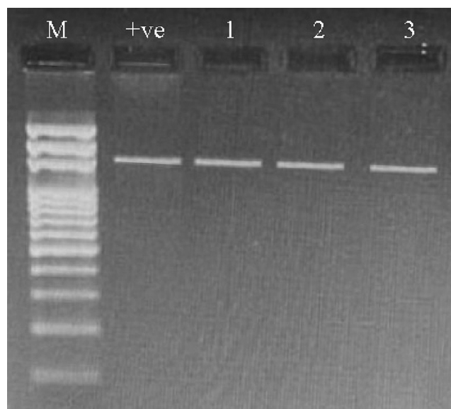
Fig. 5. Agarose gel after loading the PCR products of 16S rRNA gene (Lanes 1–3). M: DNA marker, + ve positive control.
