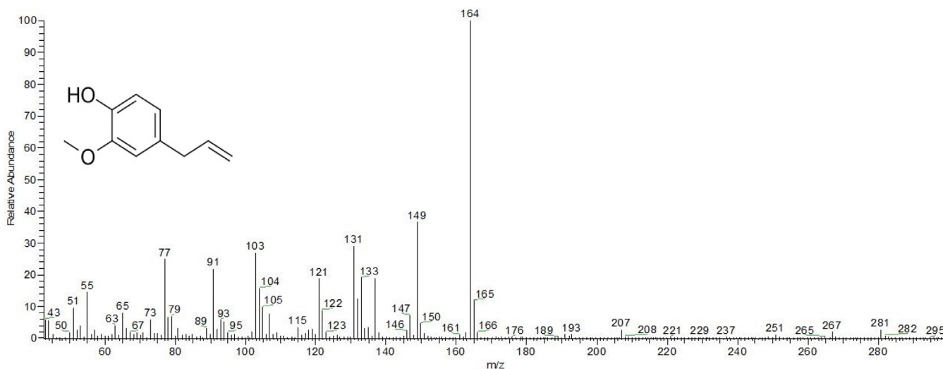
Fig. 3. Mass spectrum and chemical structure of eugenol compound.
