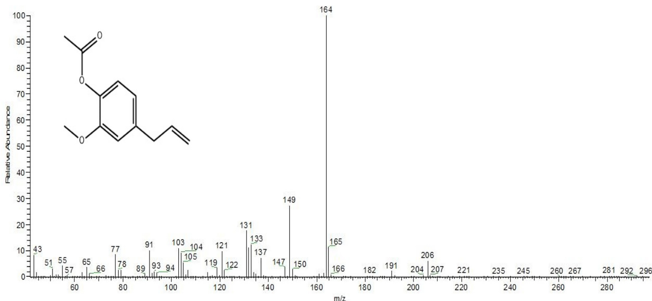
Fig. 4. Mass spectrum and chemical structure of eugenyl acetate compound.
