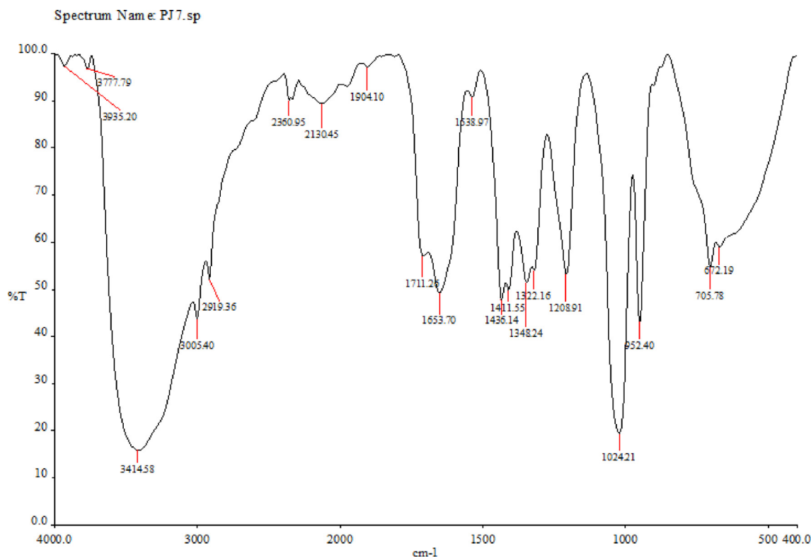
Fig. 1. FT-IR analysis of the methanolic extract of Mangifera indica seed kernels (MISK).
