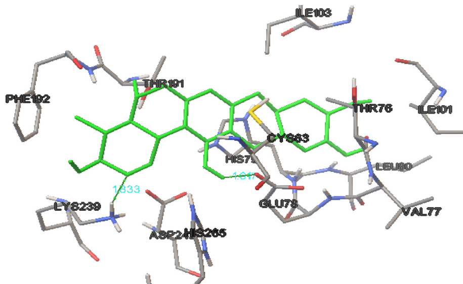
Fig. 3. The binding interaction of biofilm-producing uropathogenic E.coli LpxC protein with mangiferin.
