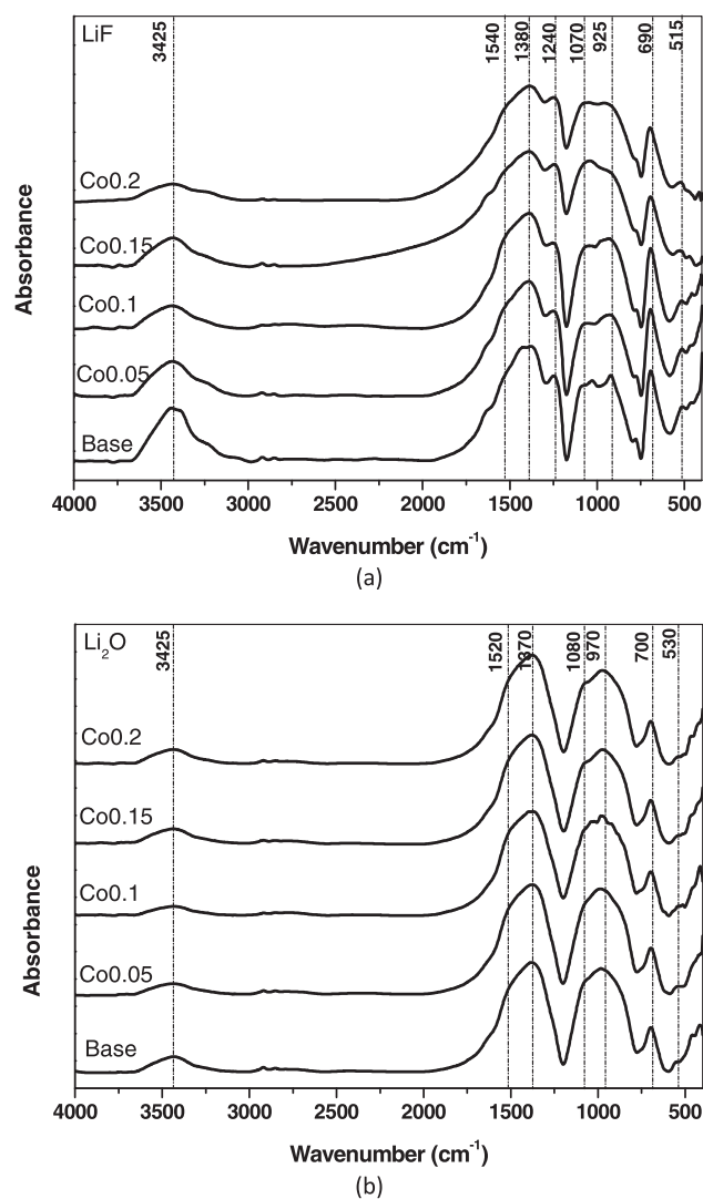
Figure 2 (a, b) FTIR spectra of CoO-doped \text{LiF-B}_2\text{O}_3 glasses and \text{Li}_2\text{O-B}_2\text{O}_3 glasses.
