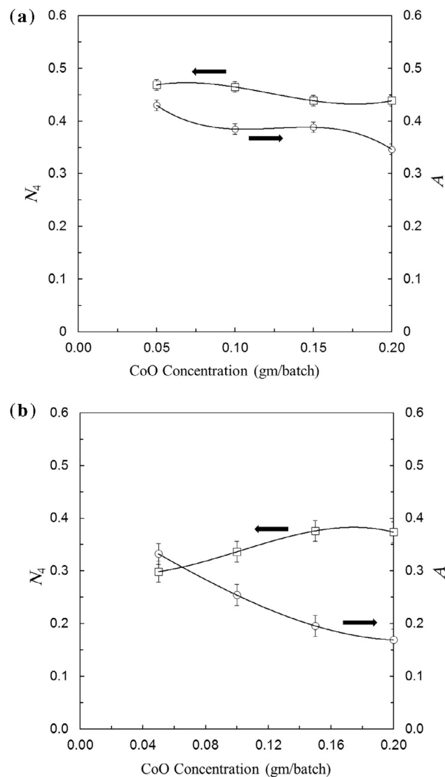
Figure 5 Calculated values of N_4 and correlation with area under visible band result from CoO both in case of LiF (a) and \text{Li}_2\text{O} (b).
