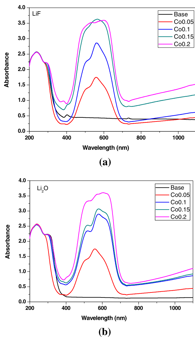
Figure 1 (a, b) Optical absorption spectra of CoO-doped LiF-B 2 O 3 and Li 2 O-B 2 O 3 glasses.
