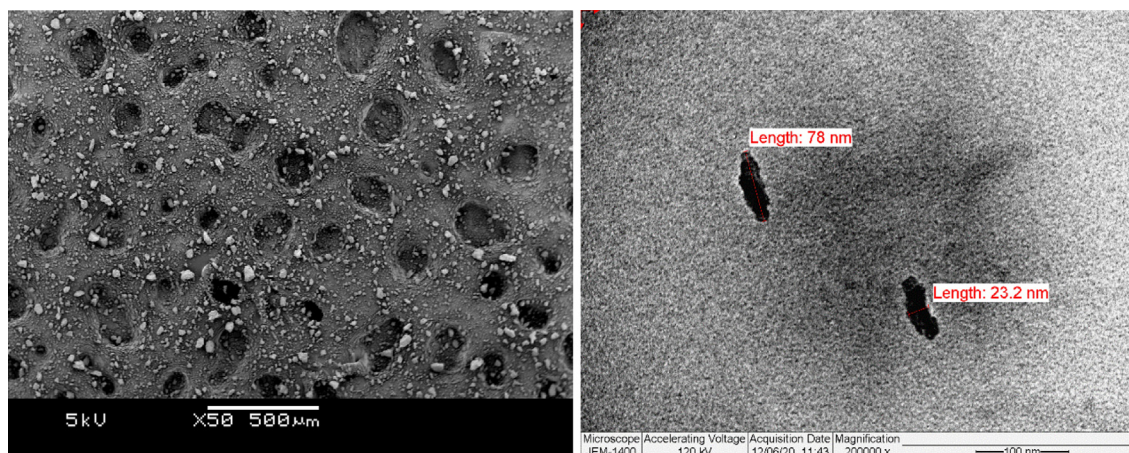
Fig. 1. SEM and TEM of date palm nanofillers (DPNF).
