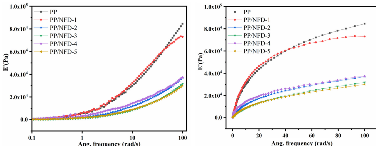
Fig. 6. Comparison of composite's storage modulus with frequency.
