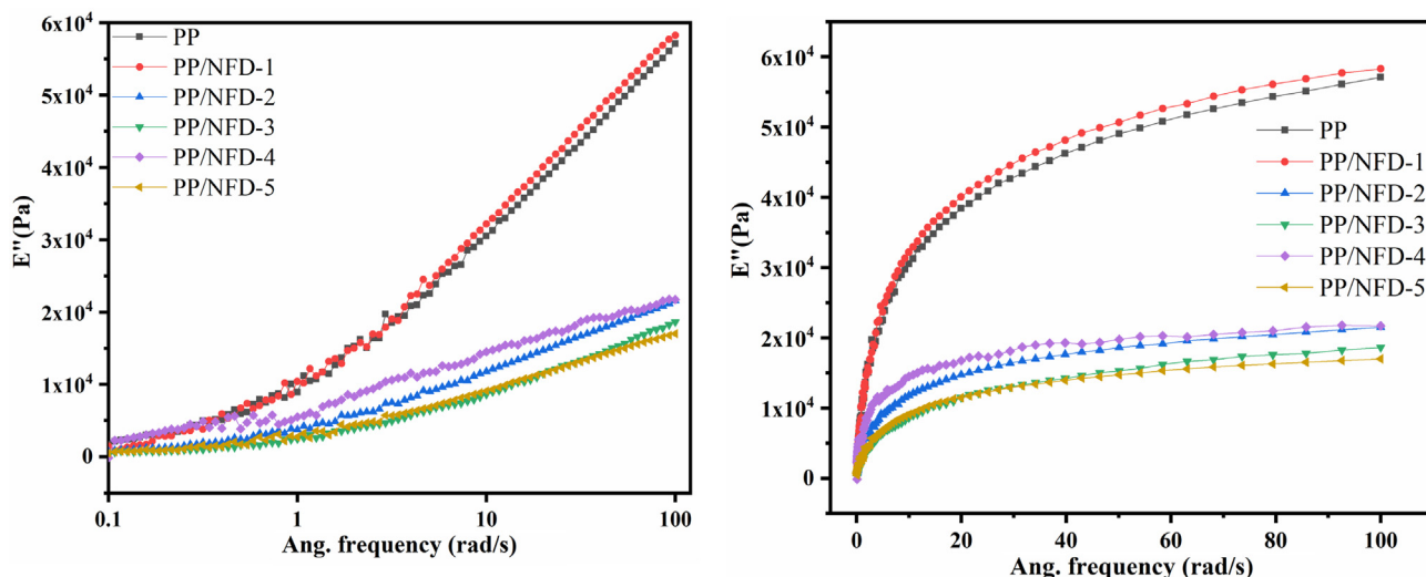
Fig. 7. Comparison of composite's loss modulus with frequency.
