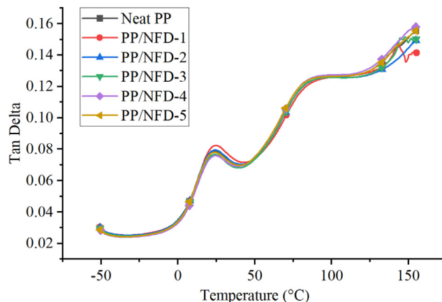
Fig. 5. Damping factor/Tan (δ) of nano date filler-based PP composite.
