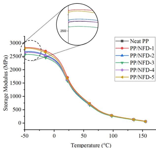
Fig. 3. Storage modulus ( E' ) of nano date filler-based PP composite.
