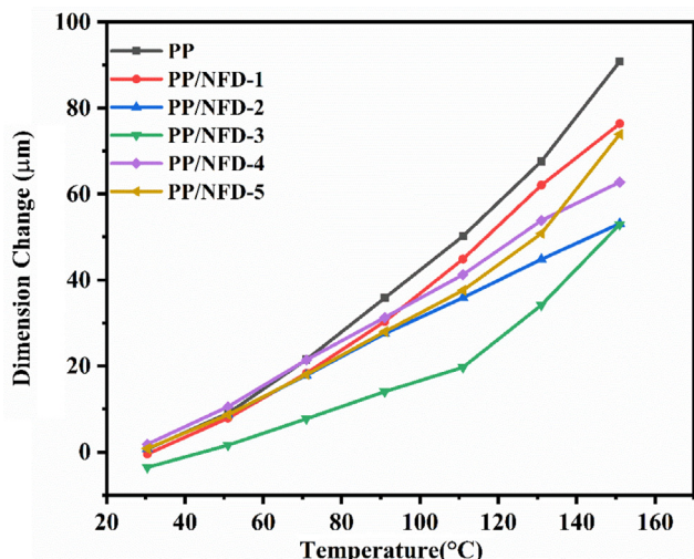
Fig. 2. Coefficient of thermal expansion (CTE) of nano date filler-based PP composite.
