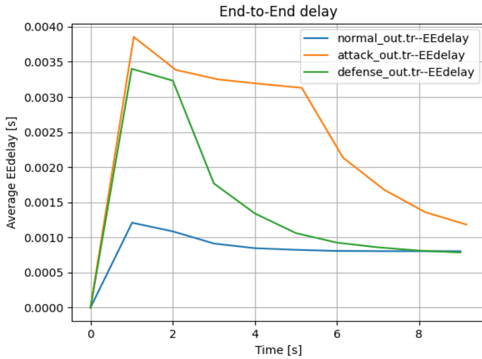
Fig. 7. Average end-to-end delay.
