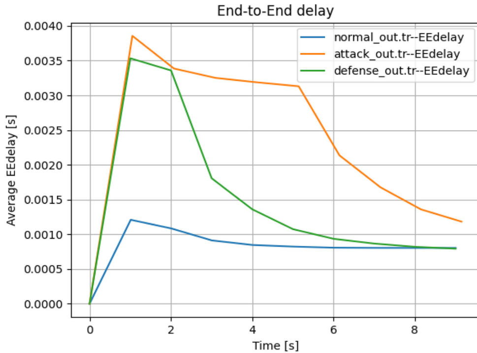
Fig. 3. Average end-to-end delay.
