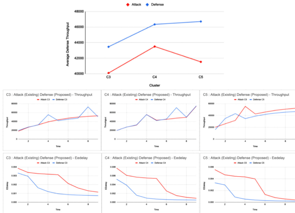
Fig. 2. Throughput difference on the application of proposed defense on the cited attack.
