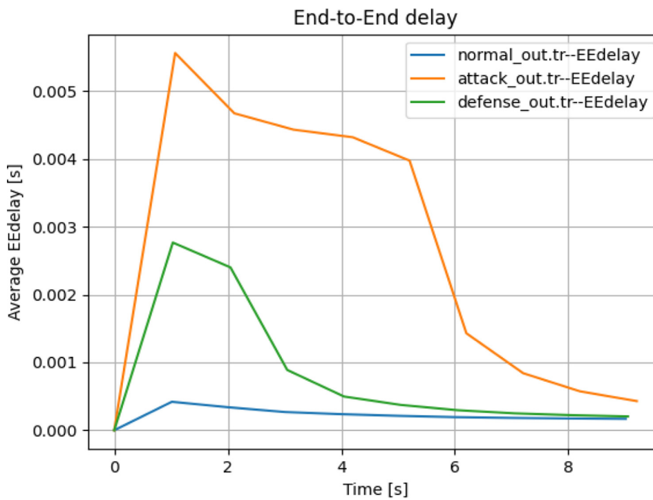
Fig. 6. Average end-to-end delay.
