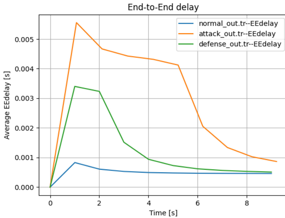
Fig. 8. Average end-to-end delay.
