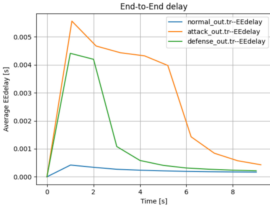
Fig. 5. Average end-to-end delay.
