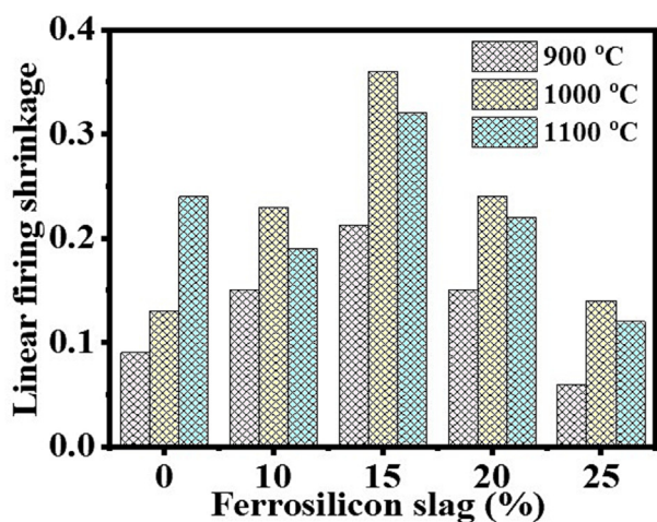
Fig. 5. The influence of FS slag addition and firing temperatures on linear firing shrinkage.
