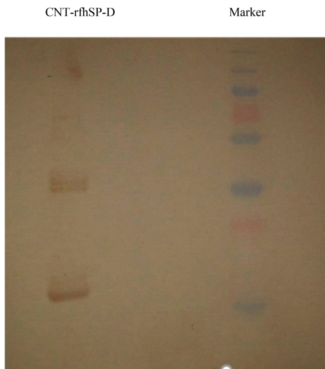
Fig. 2. Binding of rfhSP-D to CMC-CNT. Analysis of rfhSP-D with 12% wt/vol SDS-PAGE solution. CMC-CNTs were incubated overnight along with purified rfhSP-D, in a weight ratio of 1:2. They were washed with PBS afterwards and then put into a centrifuge to remove all free rfhSP-D. The first lane in the figure shows the molecular weight marker, while the second lane shows CMC-CNT – rfhSP-D. Monomeric, dimeric, and trimeric protein chains can also be seen in lane 2.
