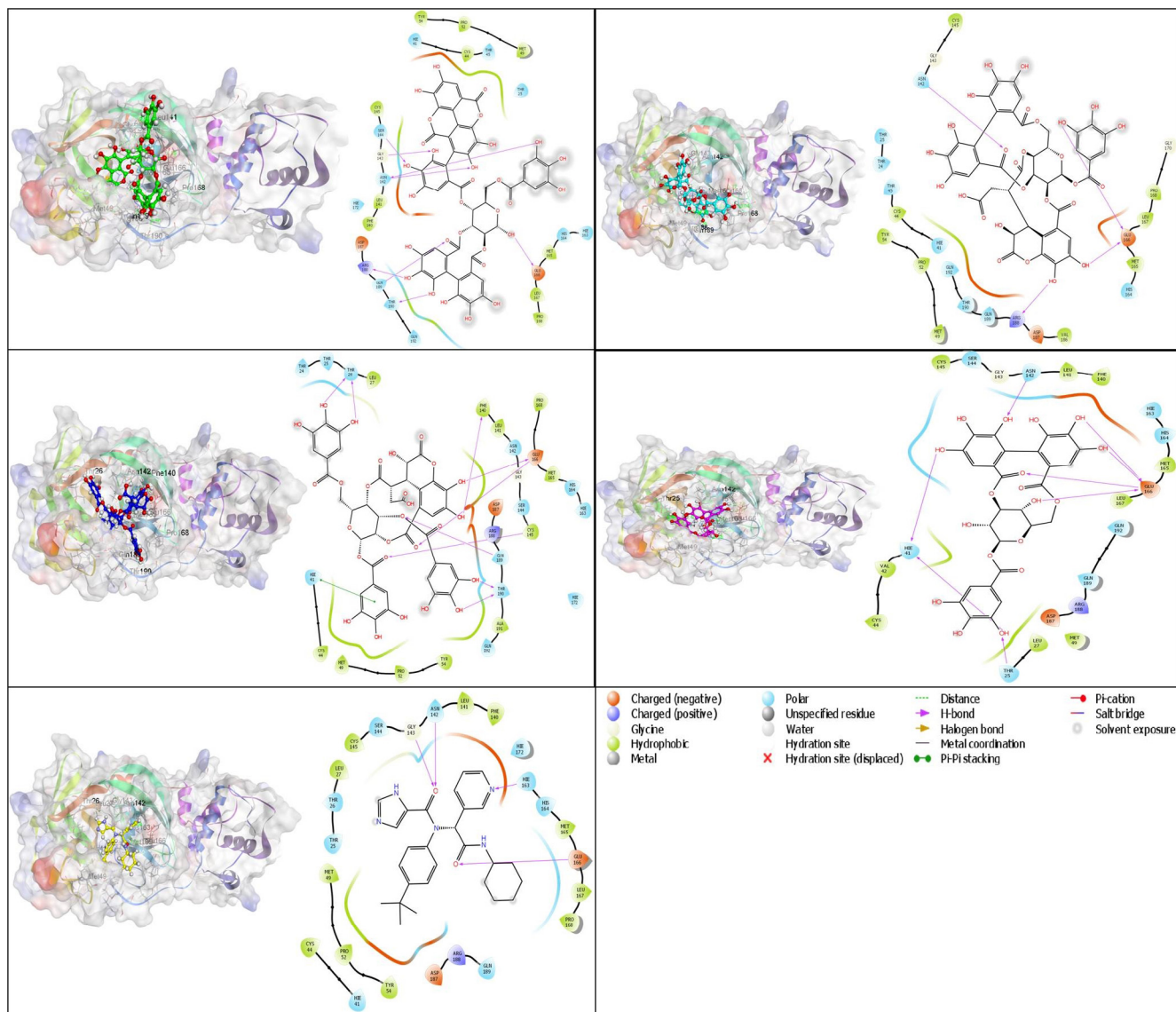
Fig. 3. Interaction between the ligands and main protease ( M^{P^ro} ) (PDB: 6W63). (a) Terflavin, (b) Chebulagic acid, (c) Chebulinic acid, (d) Corilagin, (e) X77 or N-(4- tert -butylphenyl)-N-[(1R)-2-(cyclohexylamino)-2-oxo-1-(pyridin-3-yl)ethyl]-1H-imidazole-4-carboxamide.
