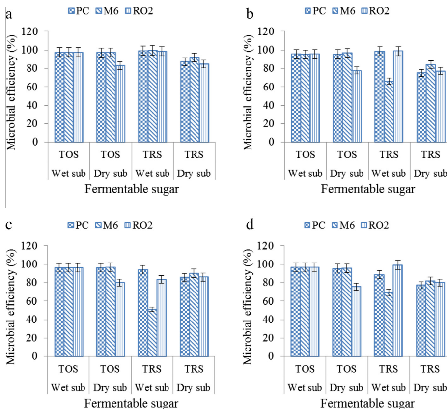
Figure 4 Substrate fermentable sugar (TOS and TRS) utilization efficiency of WRF on composite substrates (a) BpPApPp, (b) BpPAp, (c) PApPp and (d) BpPp.
