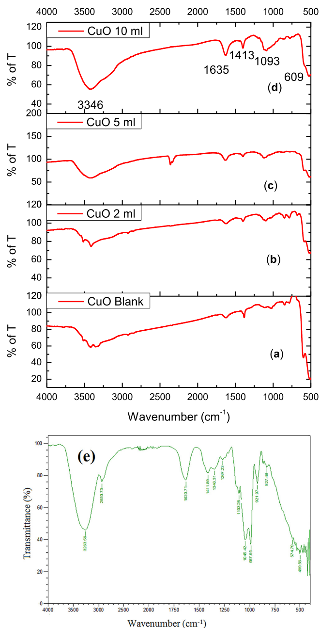
Fig. 1. (a–e). FTIR spectra (a) CuO NPs (b) CuO NPs with 2 ml (c) CuO NPs with 5 ml (d) CuO NPs with 10 ml juice (e) FTIR spectrum of sugarcane juice.
