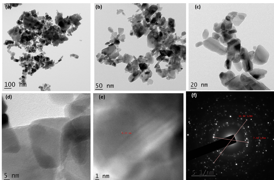
Fig. 4B. (a-f). TEM images and SAED pattern of CuO with 2 ml juice.
