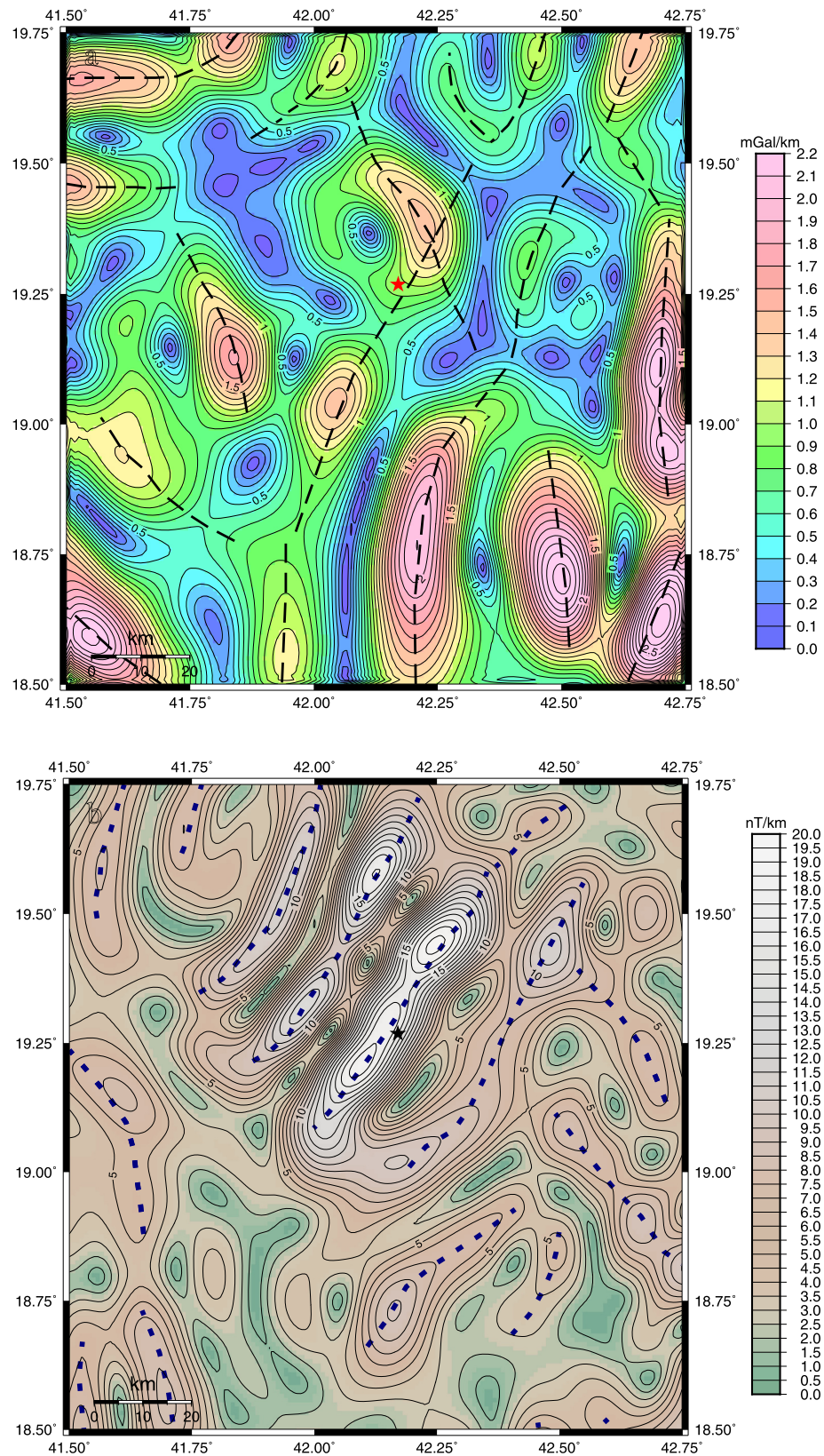
Fig. 4. (a) Map of the Magnitude of horizontal gradient (MHG) derived from the residual gravity anomalies. It shows the gravity lineaments that correspond to edge locations of density contrasts within blocks of the basement of the Arabian Shield. Contour interval is 0.1 mGal/km. (b) Map of the Magnitude of horizontal gradient (MHG) derived from the RTP magnetic anomalies. It shows the magnetic lineaments that correspond to edge locations of magnetic property contrasts within blocks of the basement of the Arabian Shield. Contour interval is 1 nT/km. Star refers to the epicenter of the main shock of 2017 Namas earthquake.
