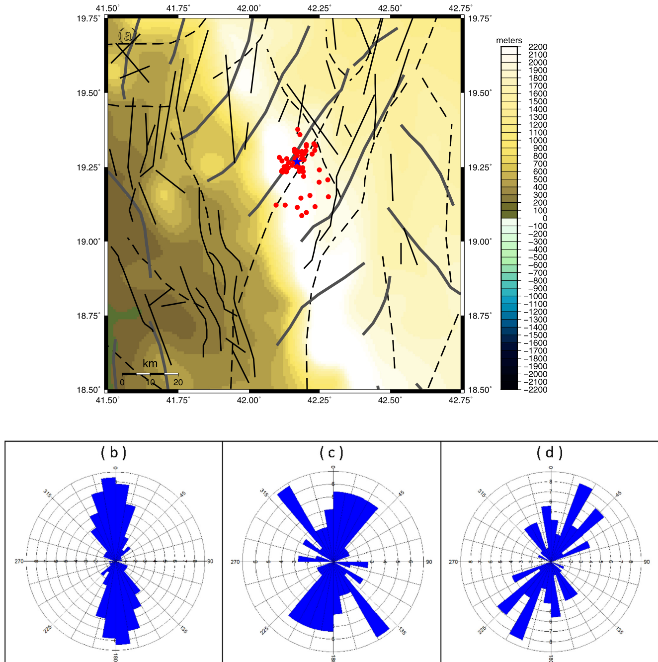
Fig. 6. (a) Structural map showing gravity and magnetic trends that were obtained from the MHG ( Fig. 4 ), surface observed faults mirrored from the geological map and seismic epicenters with magnitude higher than 2.0. Thin black lines represents surface observed faults, dashed black lines represents gravity trends shown in figure-4a, gray thick lines represent magnetic trends shown in figure-4b. The Blue star refers to the epicenter of the main shock of 2017 Namas earthquake. (b), (c) and (d) are rose diagrams showing direction frequency of surface, gravity and magnetic trends respectively.
