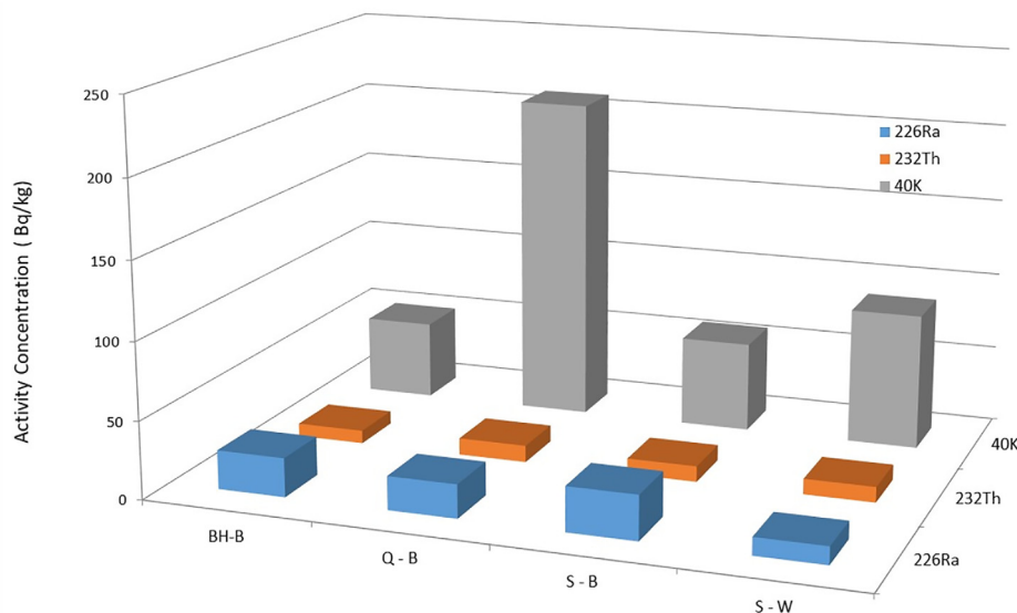
Fig. 2. Concentrations of ^{226}\text{Ra} , ^{232}\text{Th} , and ^{40}\text{K} (Bq/kg) for the cement samples.
