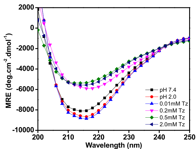
Fig 4. Far-UV CD spectra of BLG without Tz at pH 7.4 (–) 2.0 (–) and in the presence of different concentrations of 0.01 (–), 0.2 (–), 0.5 (–), and 2.0 (–) mM of Tz at pH 2.0. Tz treated samples were centrifuged several times at 10,000 rpm to remove excess dyes. The BLG concentrations were fixed 0.2 \text{ mg ml}^{-1} in every sample.
